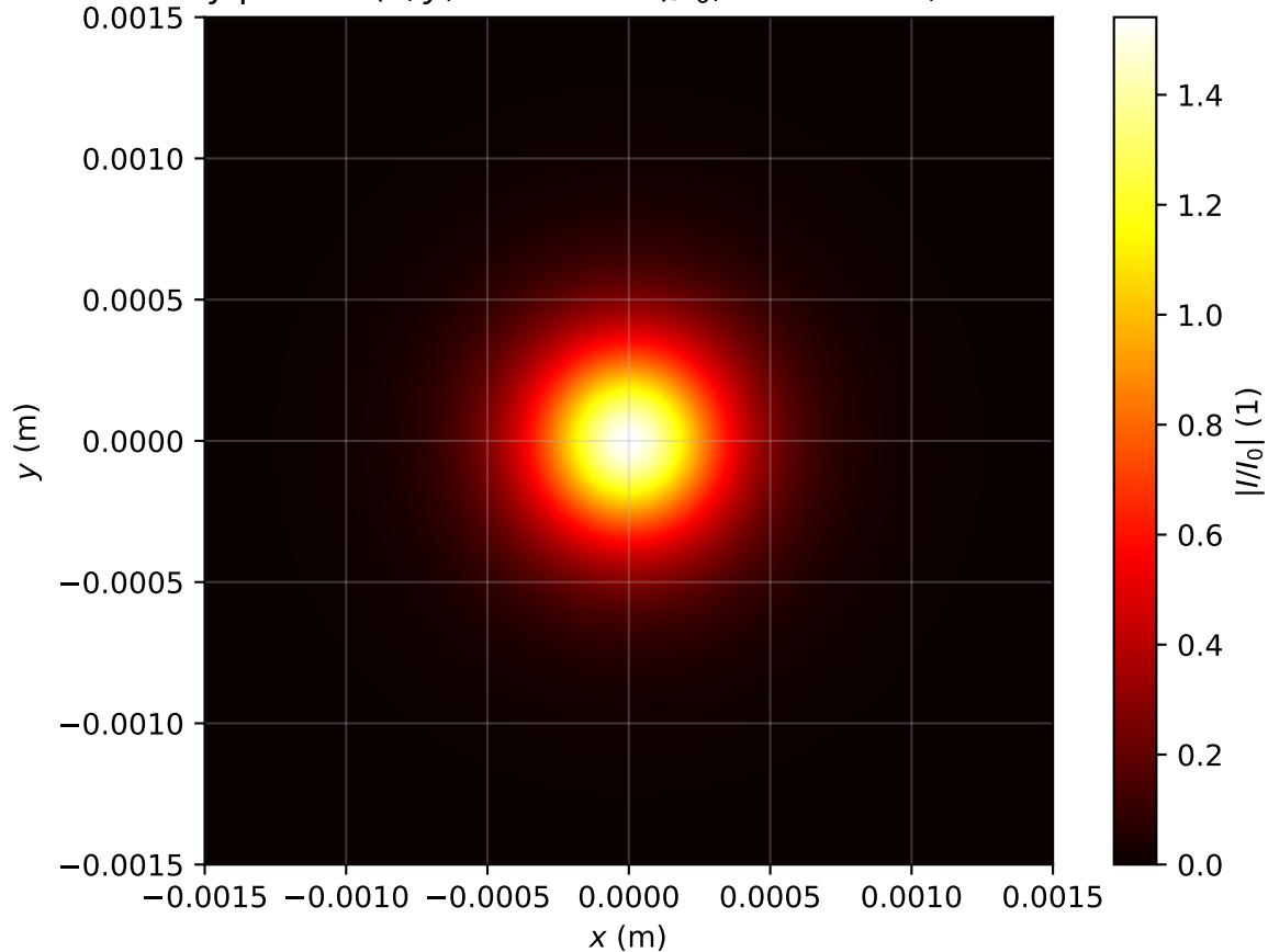
Intensity profile I(x, y, z = 3.184m)/I_0 , \text{Pin}=0.9\text{Pcr} , artificial time
